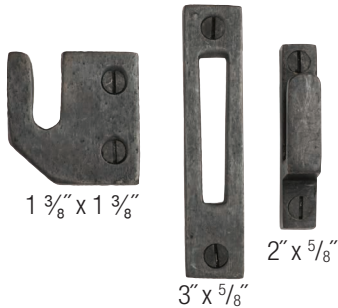
Three strike plate included with all casement fasteners
