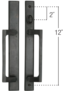
13 3/4" x 1 1/4" Plate Shown with Dunn Pull
